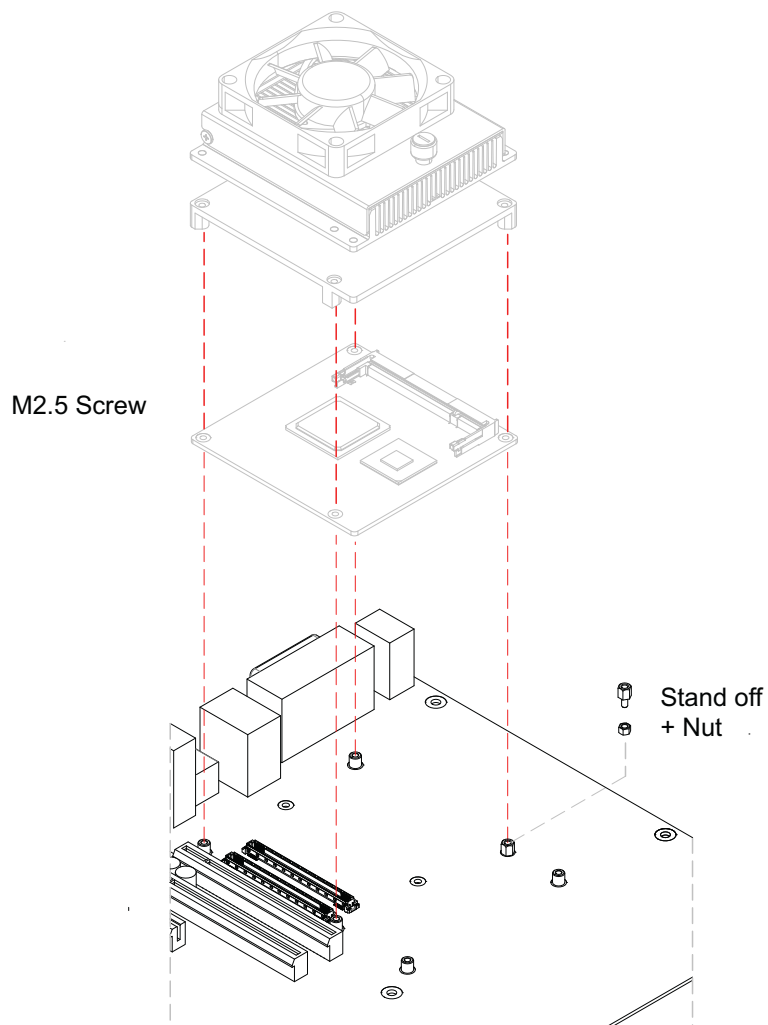
Figure 2.6 Assembly Drawing
