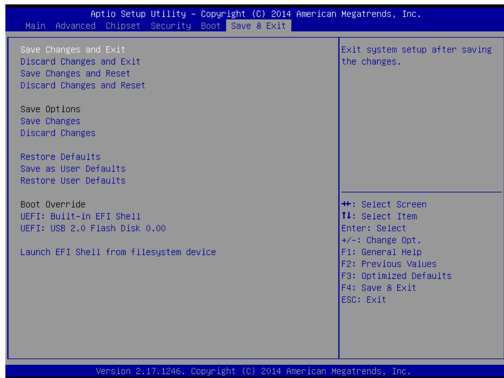
Figure 3.36 Save & Exit
