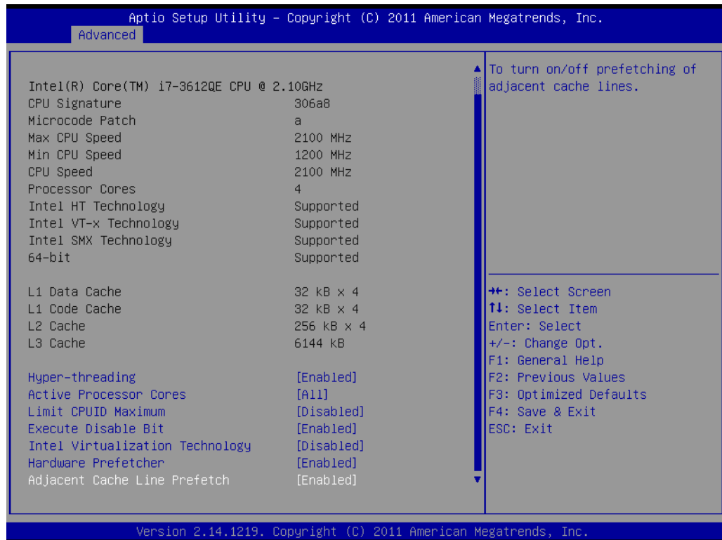
Figure 3.7 CPU Configuration
