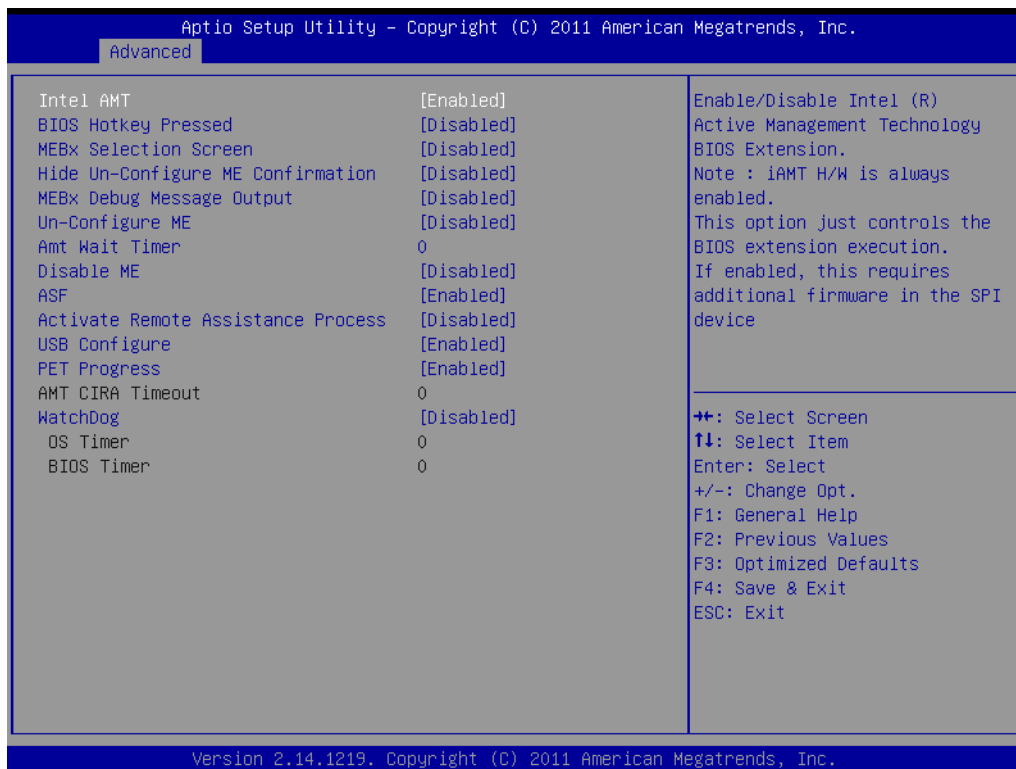
Figure 3.14 AMT Configuration
