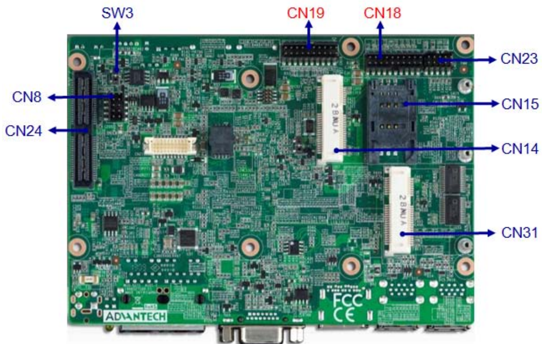
Figure 2.2 MIO-5271 Connector Locations (Bottom Side)
