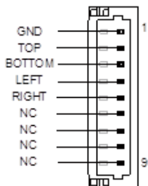
4-Wire Mode
