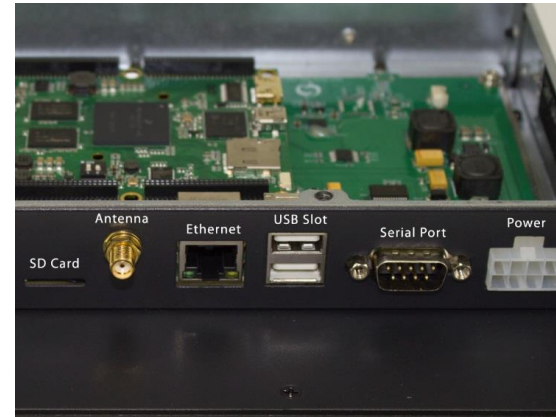
Figure 3: Side View
