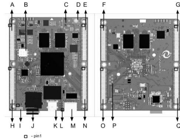
Figure 2: HIO-EMB-1200 Core Board
