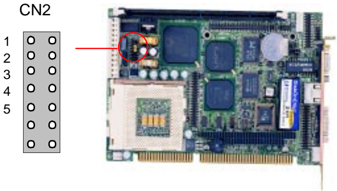
IrDA connector (CN2, Pin1 ~ 5)
