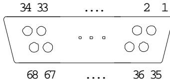
SBC-599 Wide SCSI connector (CN6)
