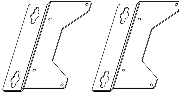
Fig. 23: Left/right mounting bracket for wall / table mounting
